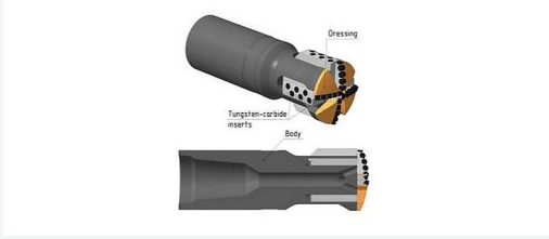
Junk mills
