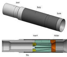
Fishing tools
