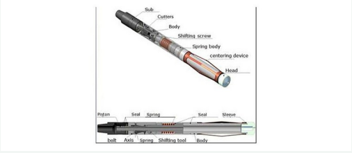
Pipe cutters
