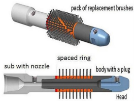
Wellbore cleaning
