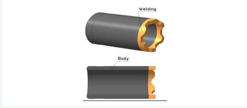
Washover shoes
